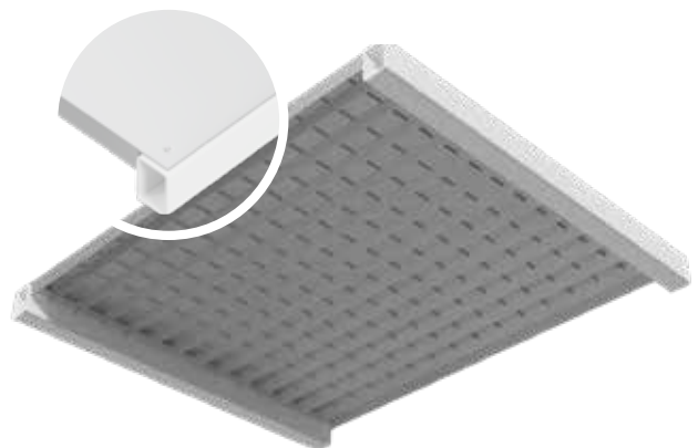
Rack grating with steel plate as a heat sink
