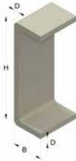
U-section
