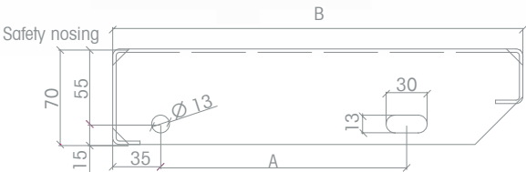
HOLE PATTERN 1
