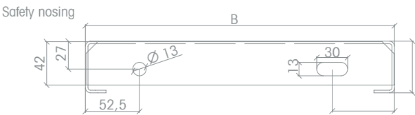
HOLE PATTERN 2
