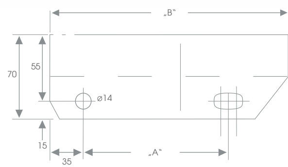
HOLE PATTERN
